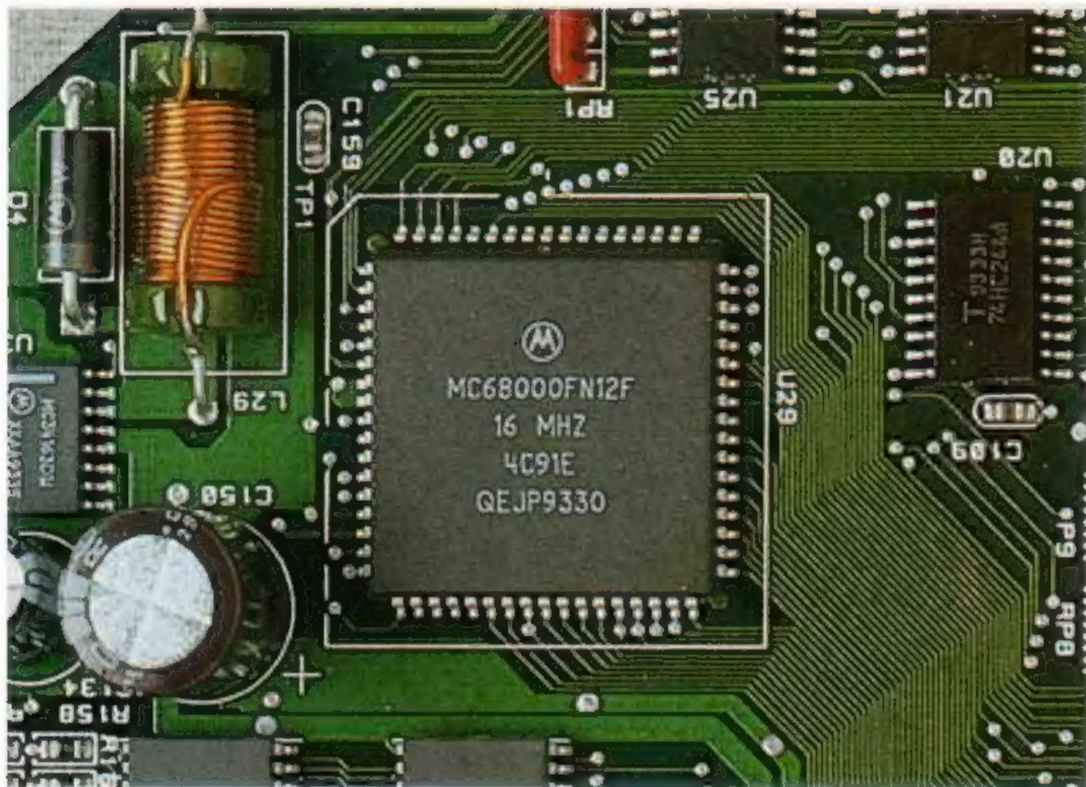
While the Jaguar has a 64bit multiprocessor architecture, it uses a much slower Motorola MC68000 to take control of the chipset
